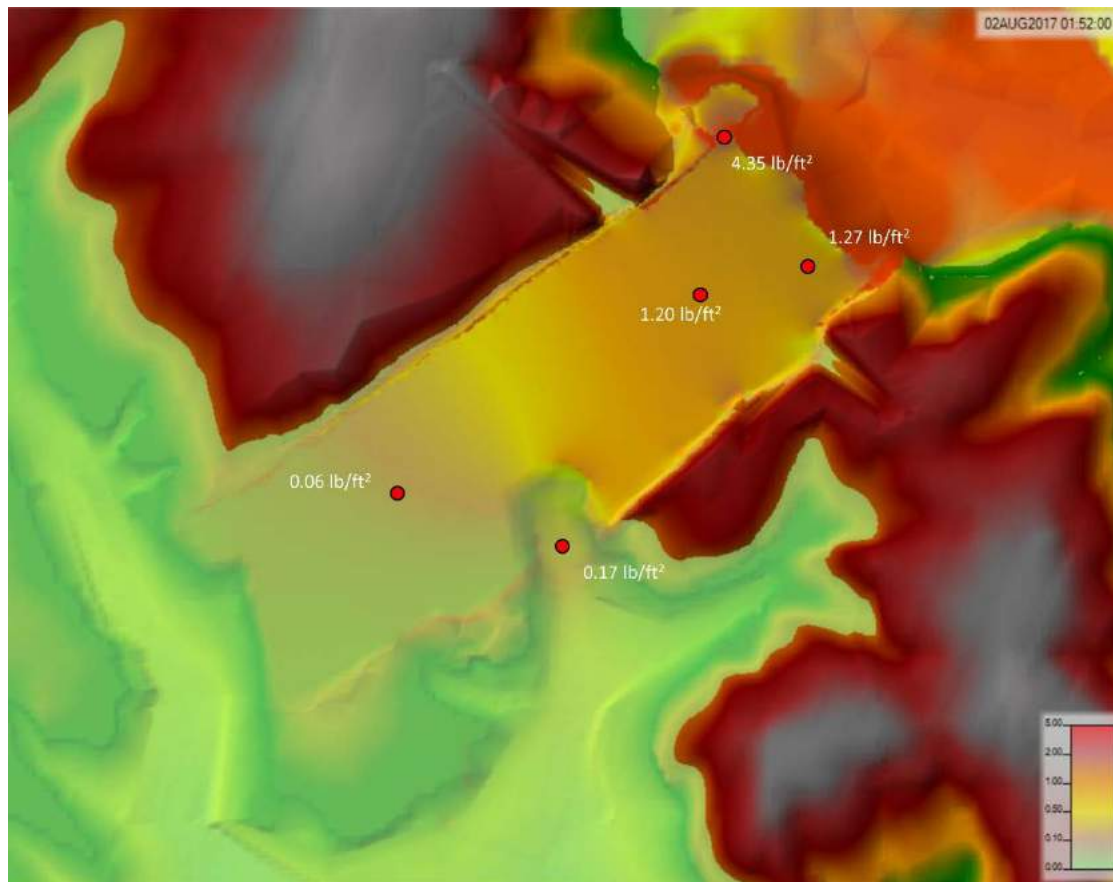
Figure 45: Shear stress color contours (lb/ft 2 ) and point shear stress values at peak flow rate of 51,702 cfs (which corresponds to maximum shear stress) for the Alternative 2 (Design) surface.
