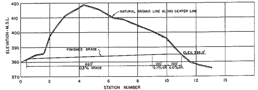
PROFILE OF EMERGENCY SPILLWAY Scale: 1"=20' Vert., 1"=200' Horiz.
