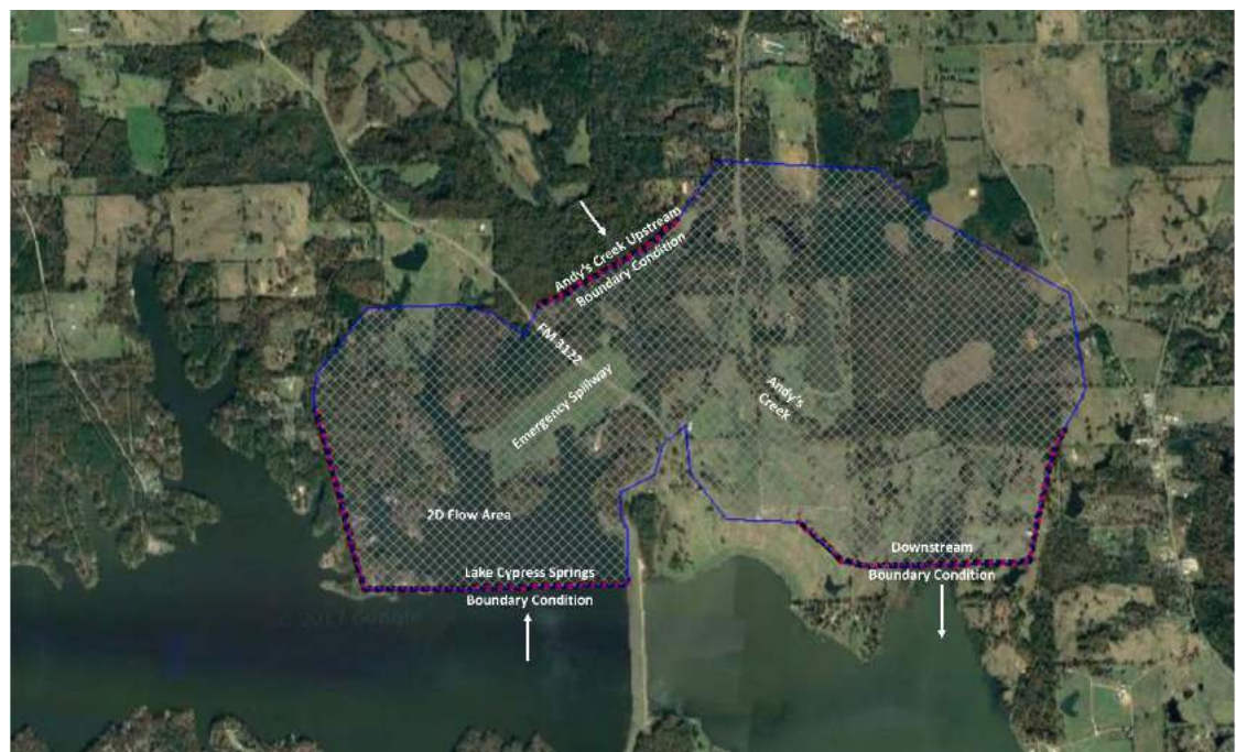
Figure 25: HEC-RAS Model Components
