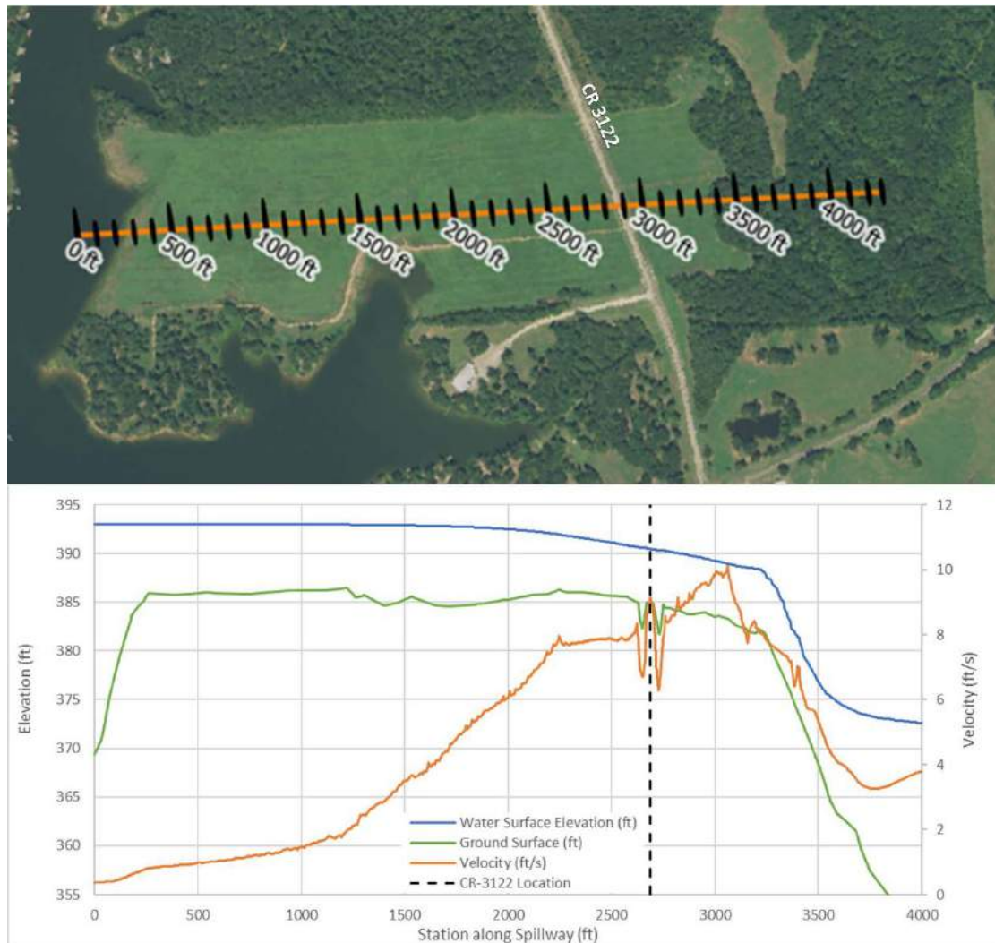
Figure 33: Andy's Creek Alternative 1 (Existing) Surface.
