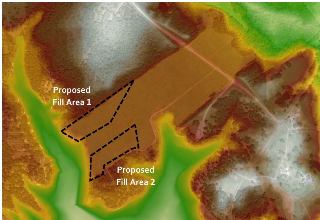
Figure 21: Proposed Locations of Fill for Alternative No. 3A (Renovated) Surface
