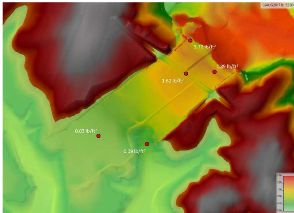
Figure 44: Shear stress color contours (lb/ft 2 ) and point shear stress values at peak flow rate of 38,418 cfs (which corresponds to maximum shear stress) for the Alternative 1 (Existing) surface.
